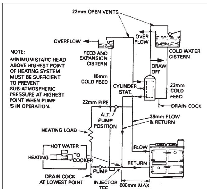
Fig. 5 Typical Central Heating/Hot Water System
