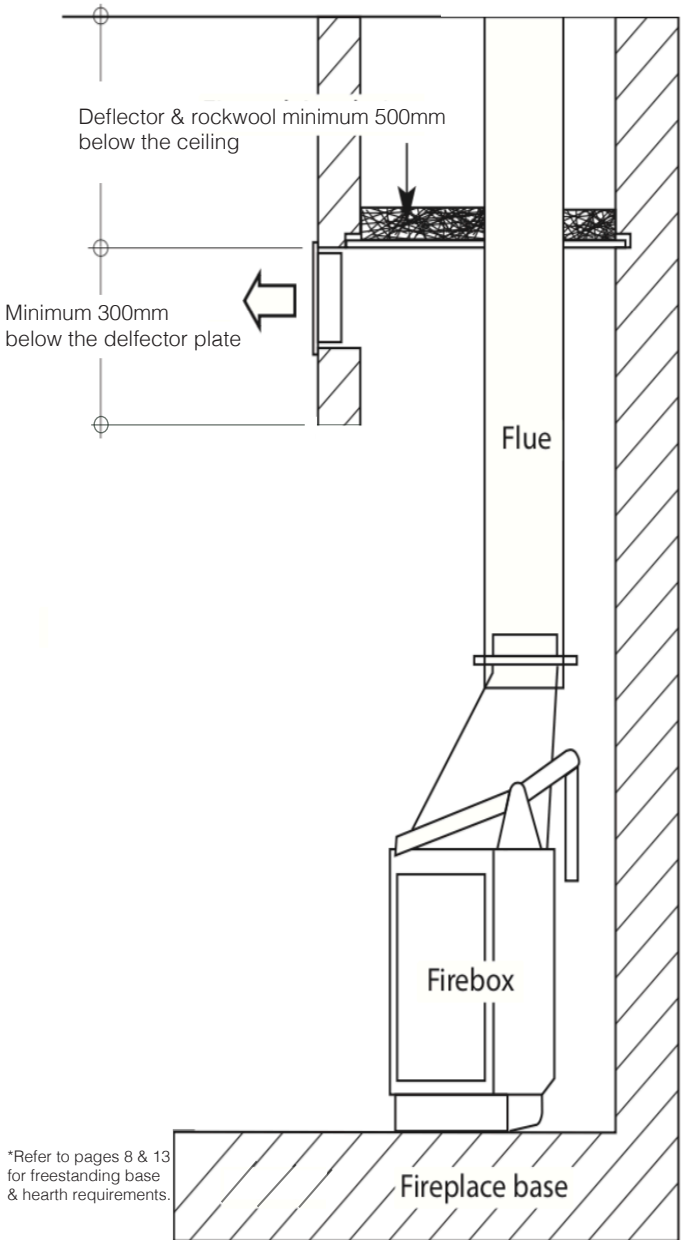
ALCOVE WITH APRON - SIDE VIEW
