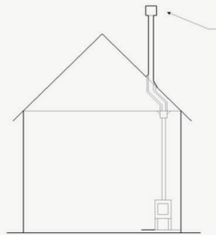
5. Flat ceiling with roof space and offset
