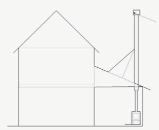
8. Double storey with single storey penetration
